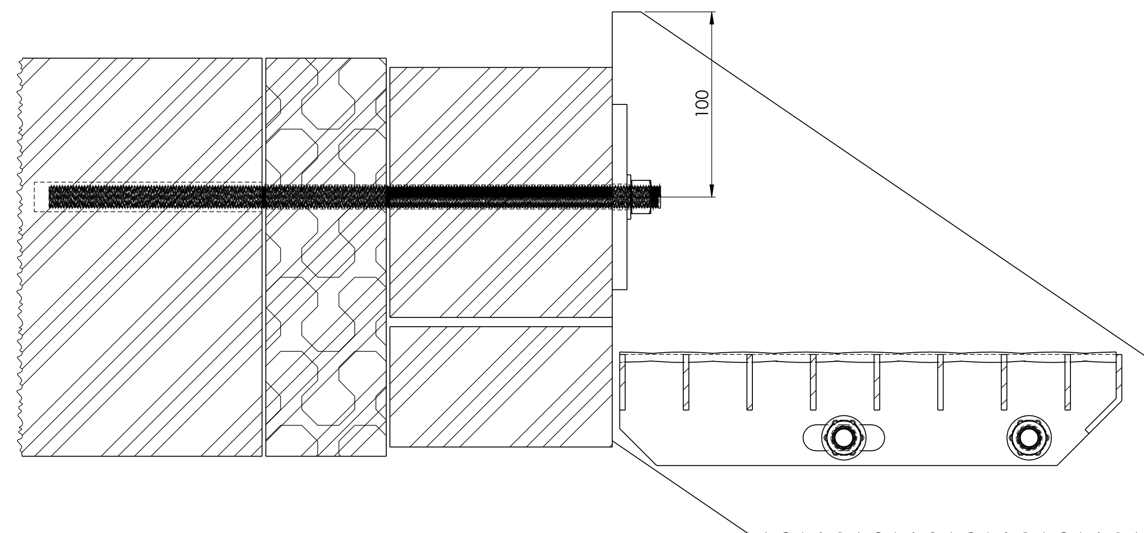
SECTION L-L
