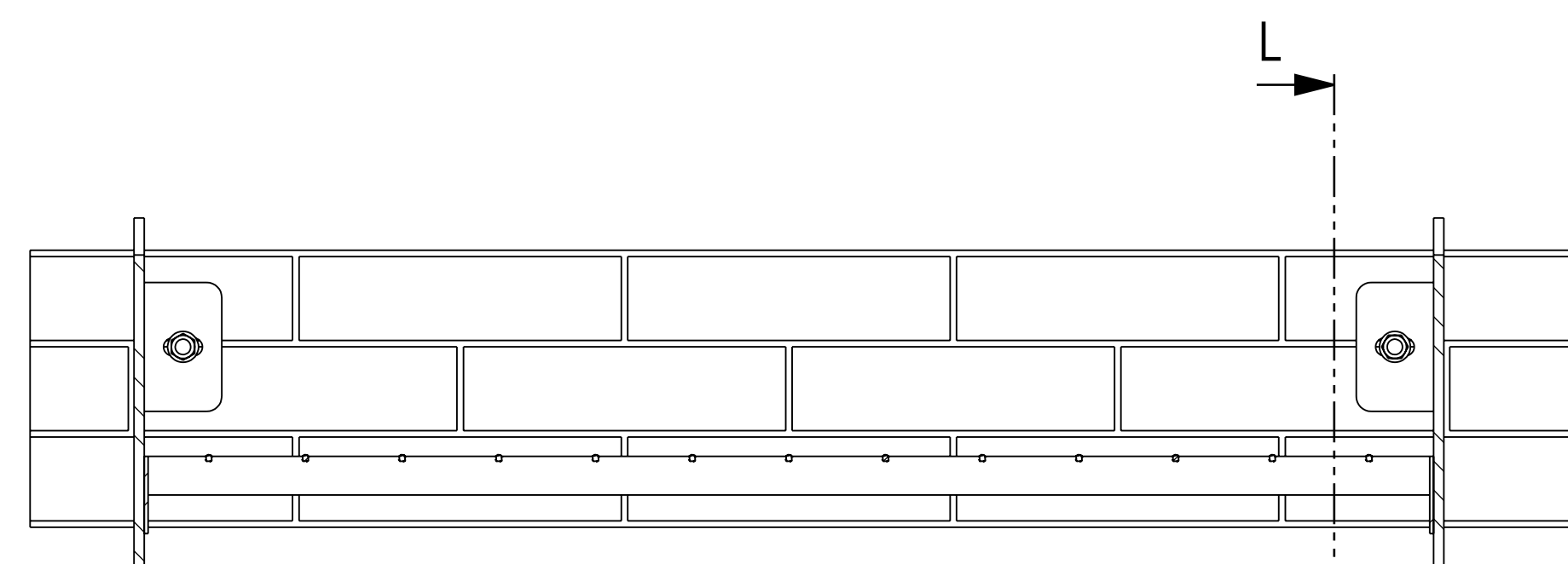
SECTION K-K
