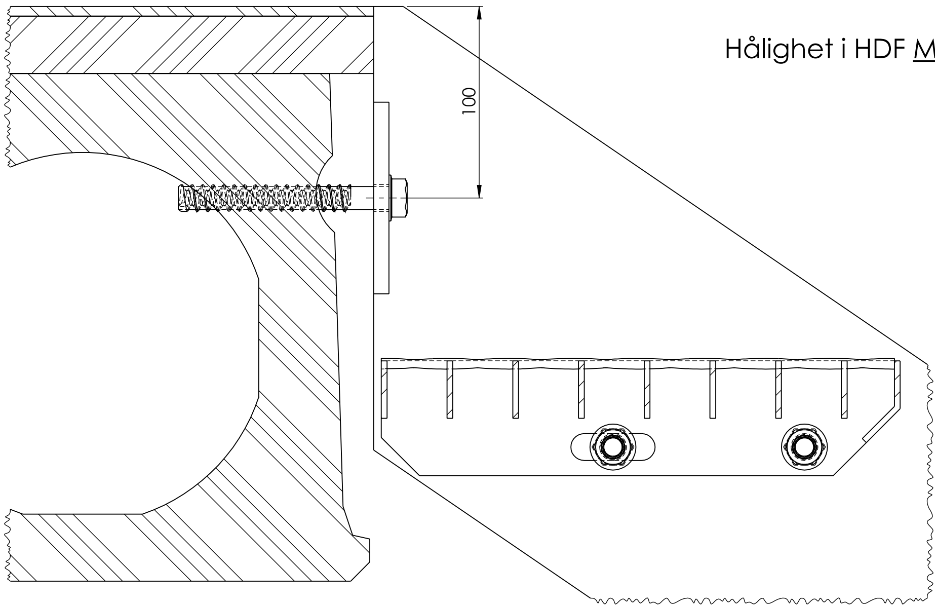
SECTION H-H SCALE 1 : 2
